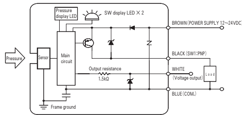
■ -PV:One PNP output and voltage output
