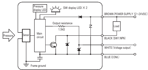
■ -NV:One NPN output and voltage output
